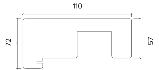
FRAME HEAD
