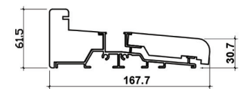
FRAME CILL
