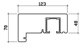
FRAME HEAD
