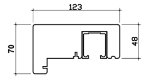
FRAME HEAD
