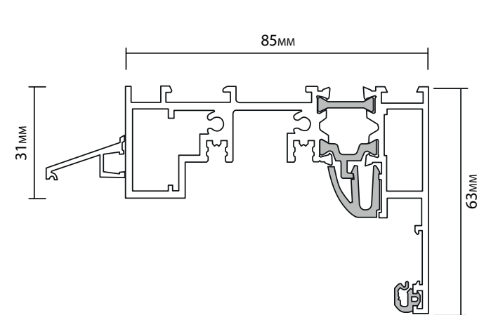
FRAME HEAD
