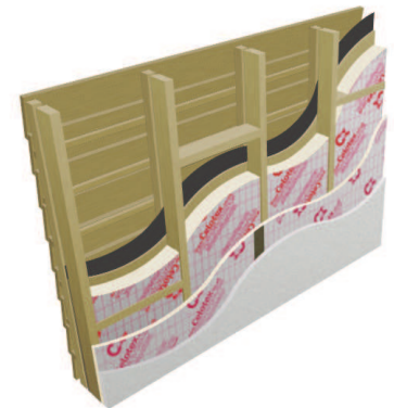
Celotex TB4000 as an internal vapour control layer, preventing thermal bridging
