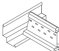
Cross Tee trimmed to shadowline T 1508 HB at perimeter
