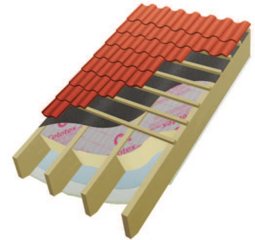
Celotex XR4000 between rafters
